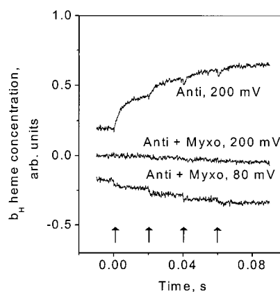
FIGURE 1: Kinetic traces of cytochrome b_H on flash excitation (arrows) of Rb. sphaeroides chromatophores. Chromatophores were suspended in buffer A with 10 \mu M PMS, and 2 \mu M methylene blue. Traces shown are the average of 4, with 10 s (top and center traces) and 50 s (bottom trace) between measurements. The redox potential was 200 mV (top and center) and 80 mV (bottom). Where indicated, the concentrations of antimycin A and myxothiazol were 7 and 2 \mu M, respectively.
